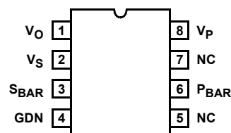
ICL7673 (SOIC, PDIP) TOP VIEW
