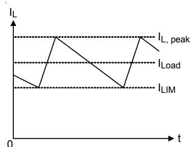
Figure 7. "Valley" Current Limit
