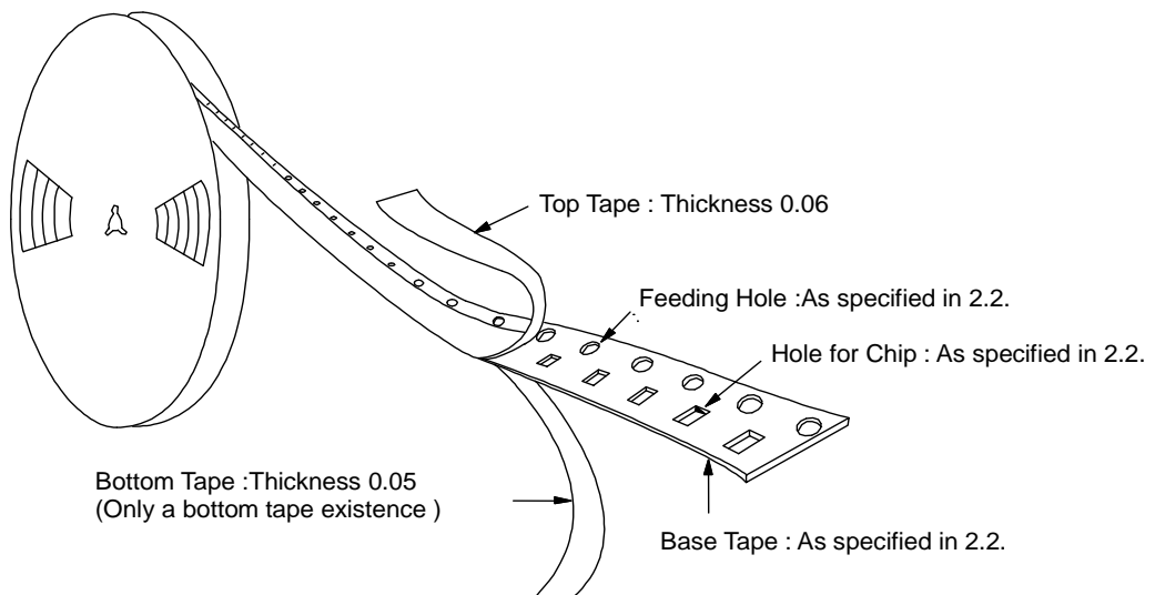
Fig.3 Taping Diagram
