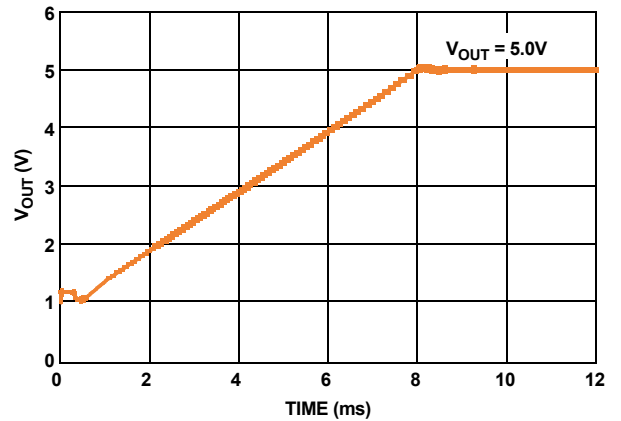
FIGURE 31. TURN-ON TIME
