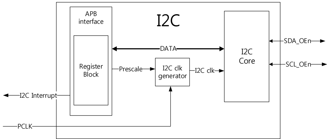
Figure 46. I2C block diagram
