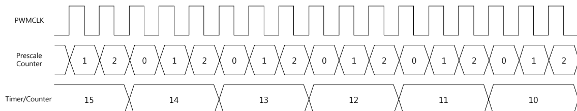
Figure 29 Down-count mode
