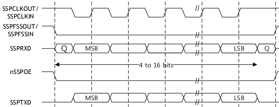
Figure 74, Q is an undefined signal.
