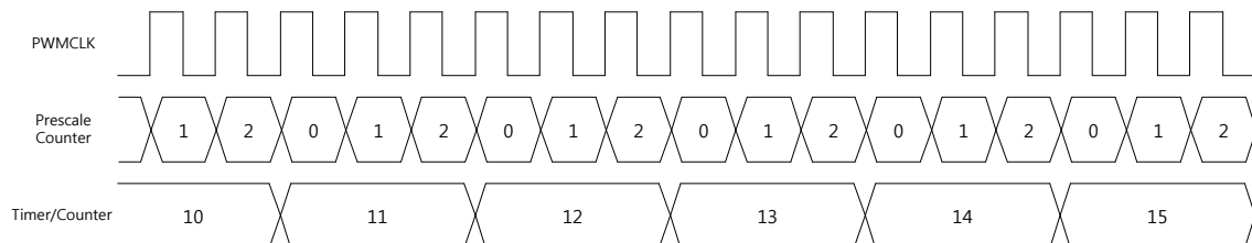
Figure 28 Up-count mode
