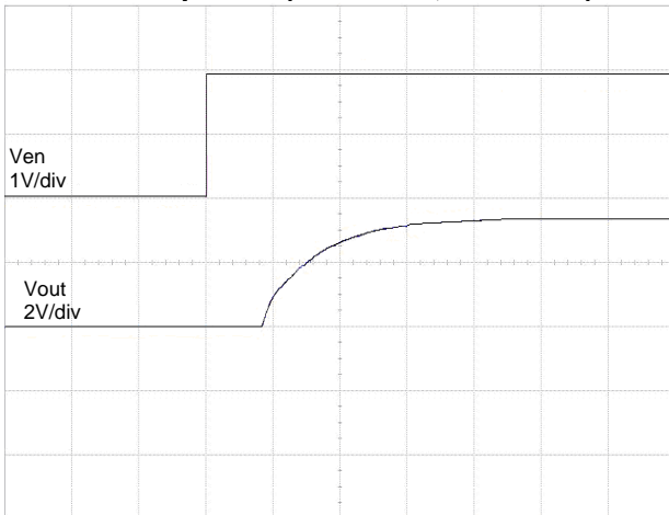
Start-up Time (Vout=3.3V, Iout=0mA)
