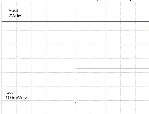
Current Limit Protection (Vout=3.3V)
