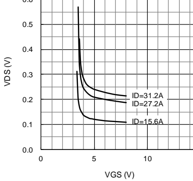
VDS-VGS characteristics (typical) Tc=25°C
