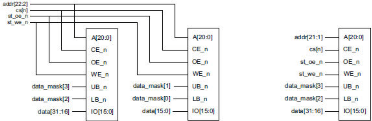
32-bit bank consisting of two 16-bit devices
